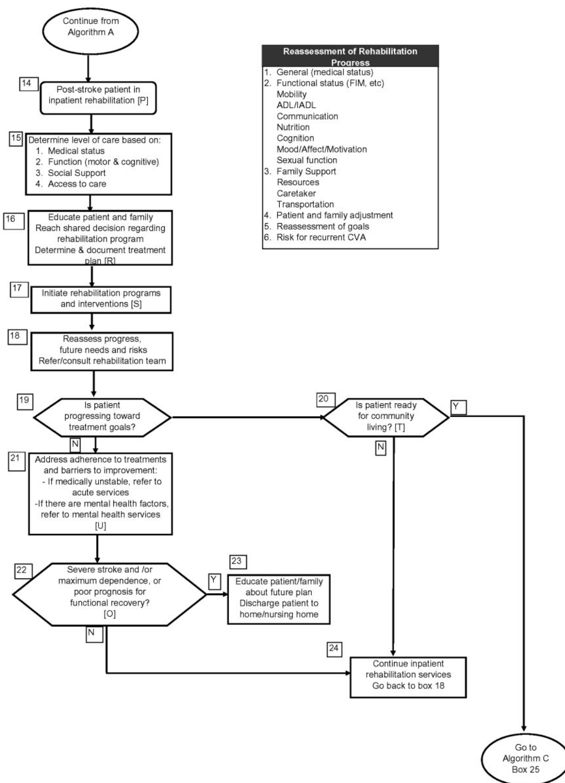
Algorithm B.
